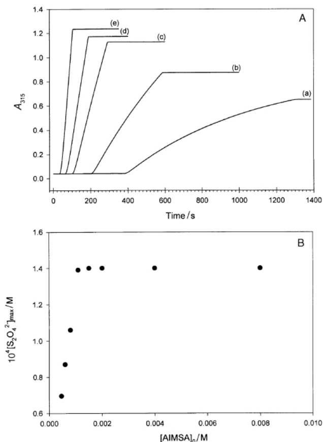
Fig. 1 (A) Formation of dithionite in the reaction of aerobic AIMSAs decomposition in 0.5 M NaOH air-saturated solution. [AIMSA] 0 = (a) 0.6 mM; (b) 1 mM; (c) 3 mM; (d) 4.6 mM; (e) 6 mM. (B) Variation of the maximum dithionite concentration formed with respect to initial AIMSAs concentrations. At high AIMSAs concentrations the limiting factor is the amount of dissolved oxygen in solution, hence the saturation is observed.
