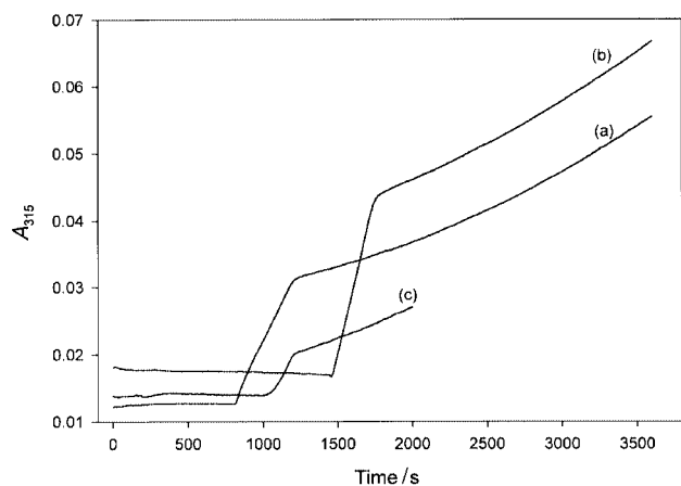
Fig. 3 Formation of dithionite during aerobic decomposition of 1.2 mM AIMSA in a buffer solution at pH 9.9: (a) without enzymes; (b) 1.5 \mu M SOD; (c) 0.125 \mu M catalase.
